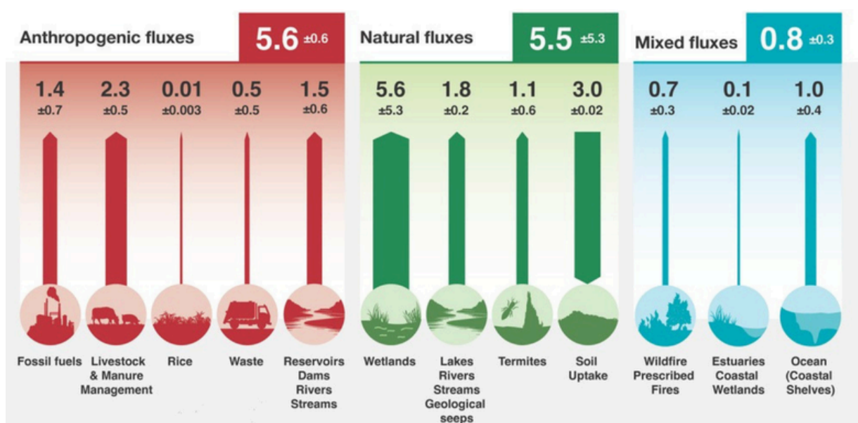
Figure 1: The methane budget for Australia (2010-2019), separated into human-caused and natural sources and sinks. Numbers are the decadal mean annual fluxes with uncertainties based on Villalobos et al. 2025.
